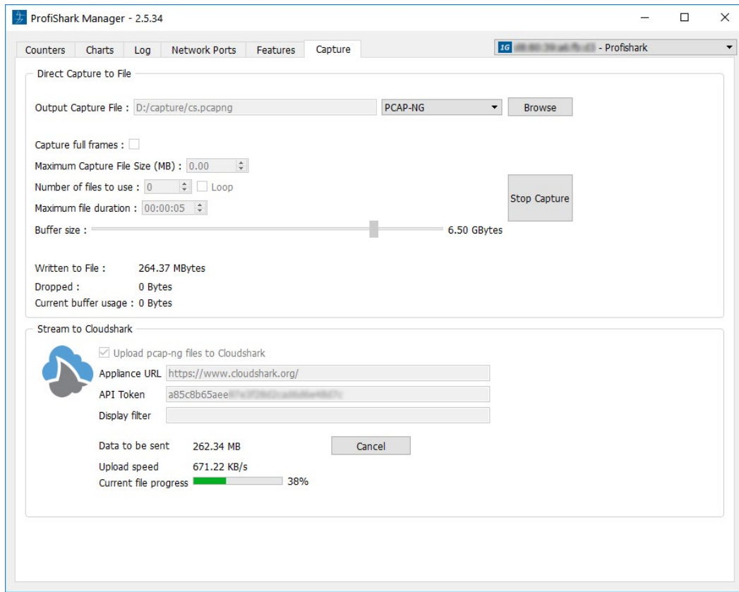
ProfiShark Manager with CloudShark integration.
